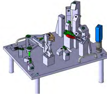
Housing gauge for automotive lighting
