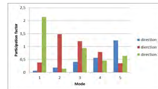
Participation factor for first six modes
