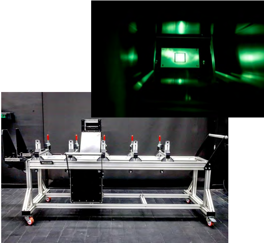
Test stand for testing and adjusting the light settings of railway signaling devices
