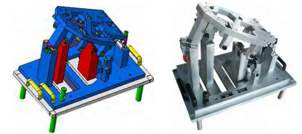
Control gauges design and production
