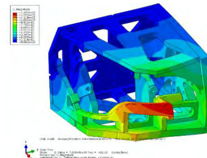
Natural frequency of holder
