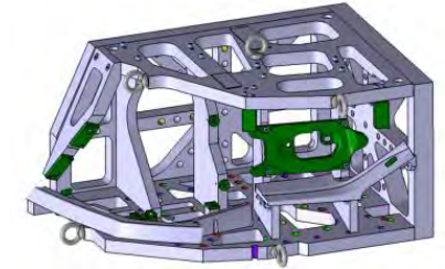
Vibration holder for lamps
