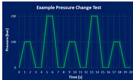
Charts: Examples of pressure change tests
