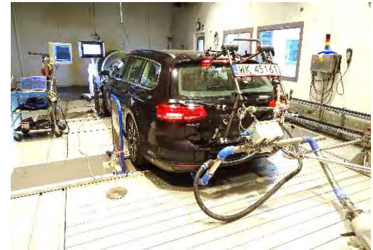
Chassis dyno verification of PEMS installation
