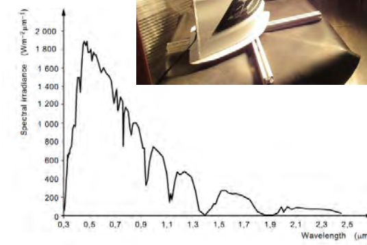
Figure 1 – Global solar spectral irradiance at sea level
