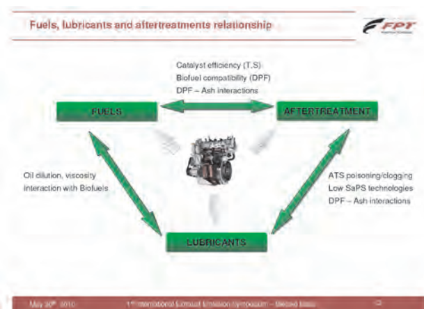
Fig. 19. Fuel-lubricant-aftertreatment interactions
