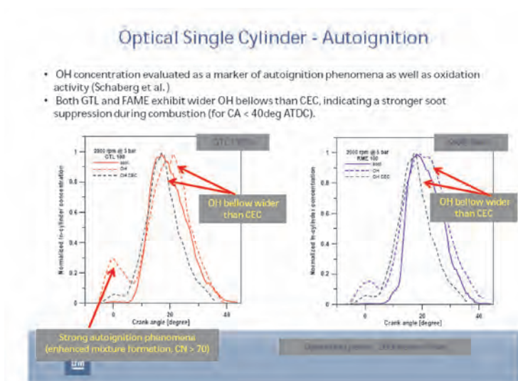
Fig. 18. Biofuel autoignition phenomena plots
