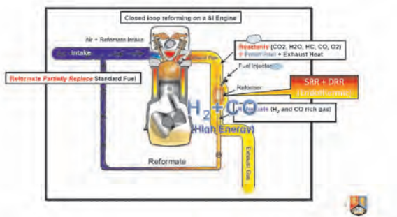
Fig. 20. Exhaust gas reformation schematic
