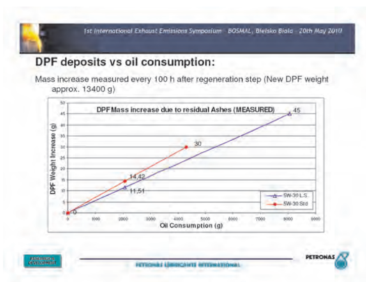
Fig. 21. DPF ash deposition results for standard and low SAPs oils
