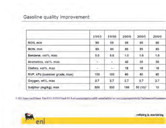
Fig. 17. Evolution of gasoline fuel quality for the EU market
